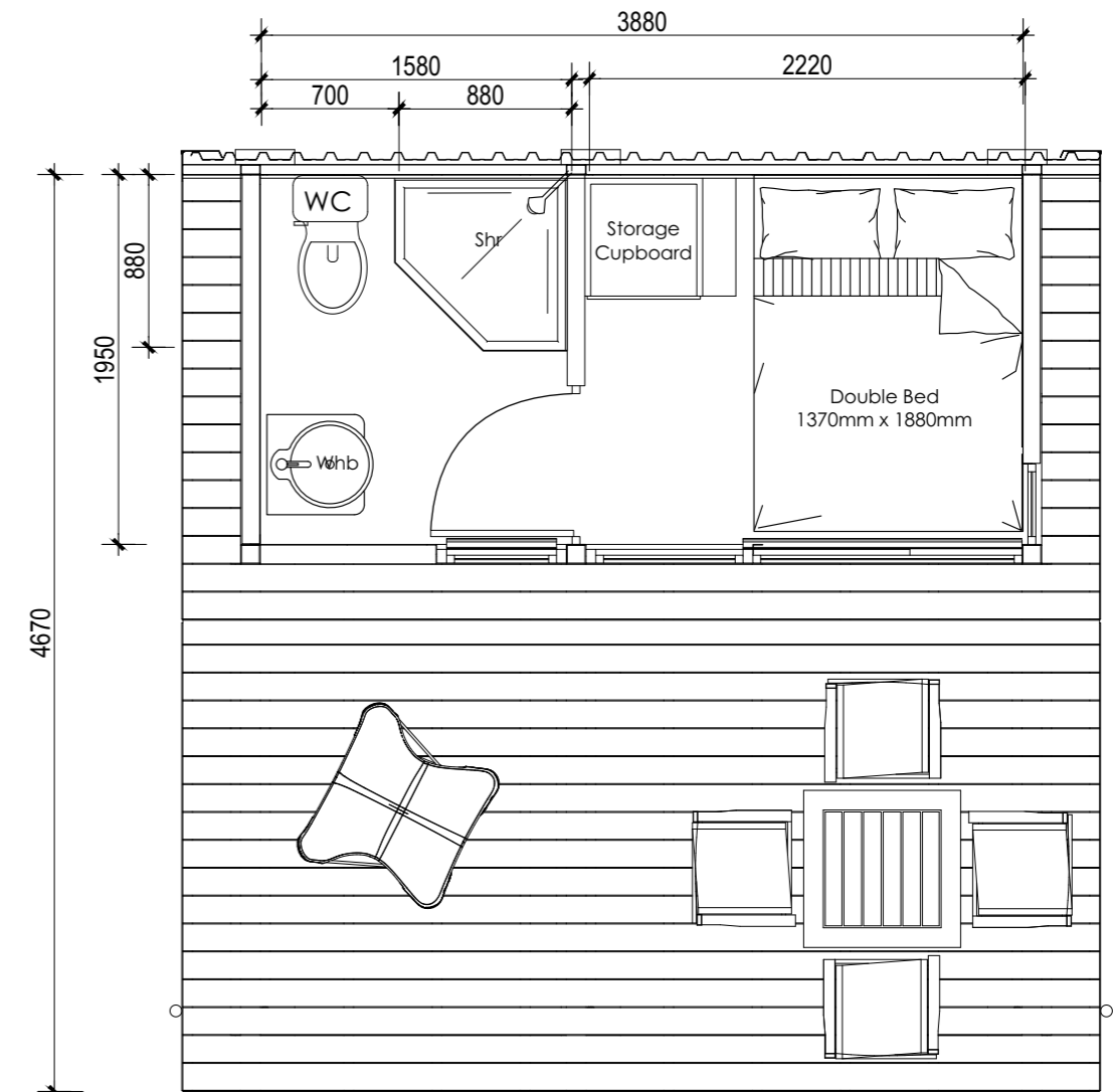
Mini Pod with Bathroom Plan Not to Scale
